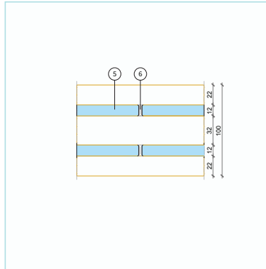
Floor connection
